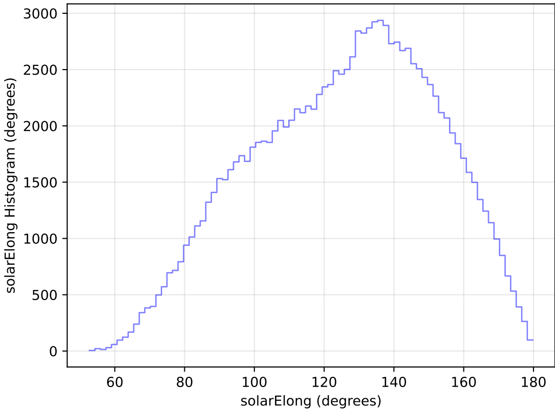
too_elab_r8_d2_griz_v3.4_10yrs All sky u band: solarElong Histogram
