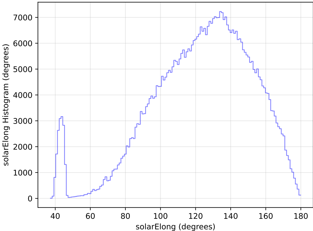
too_elab_r8_d2_griz_v3.4_10yrs All sky r band: solarElong Histogram
