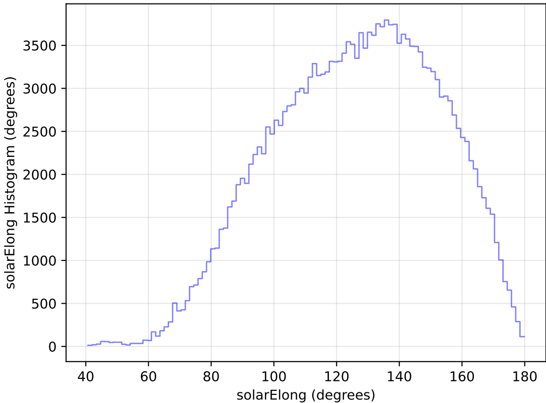
too_elab_r8_d2_griz_v3.4_10yrs All sky g band: solarElong Histogram
