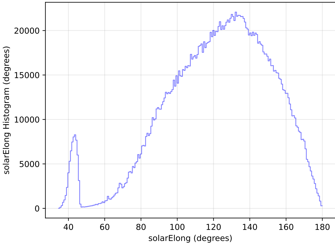
too_elab_r8_d2_griz_v3.4_10yrs All sky all bands: solarElong Histogram
