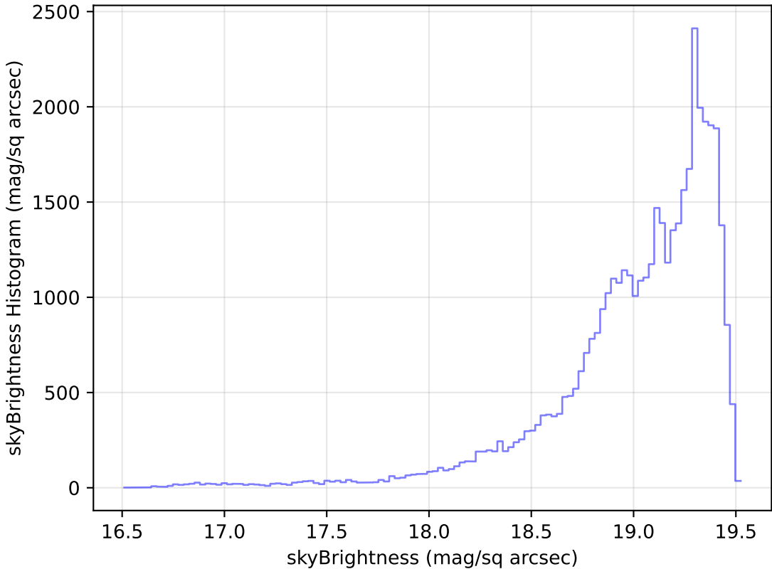
too_elab_r8_d2_griz_v3.4_10yrs Yr 1 z band: skyBrightness Histogram
