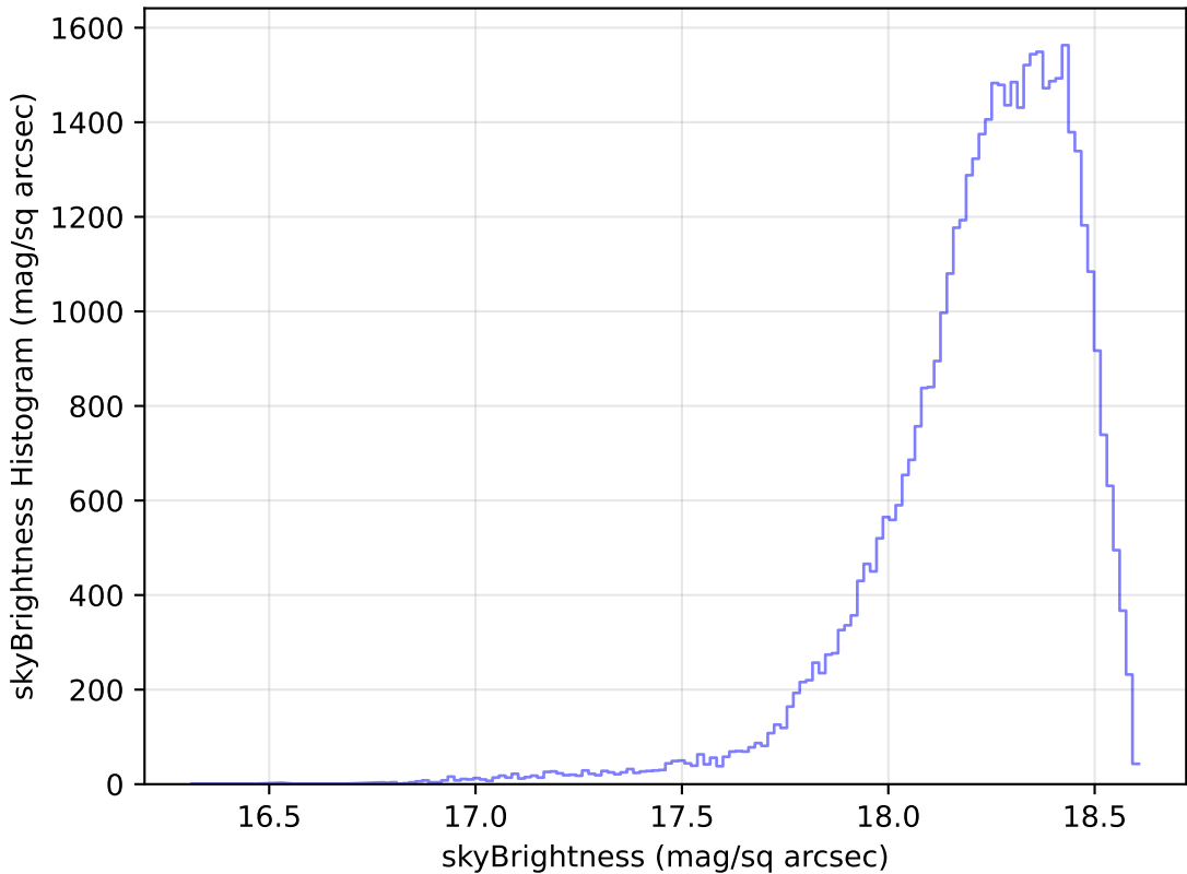
too_elab_r8_d2_griz_v3.4_10yrs Yr 1 y band: skyBrightness Histogram
