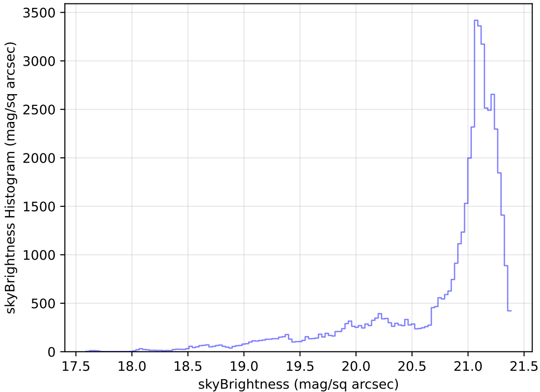
too_elab_r8_d2_griz_v3.4_10yrs Yr 1 r band: skyBrightness Histogram
