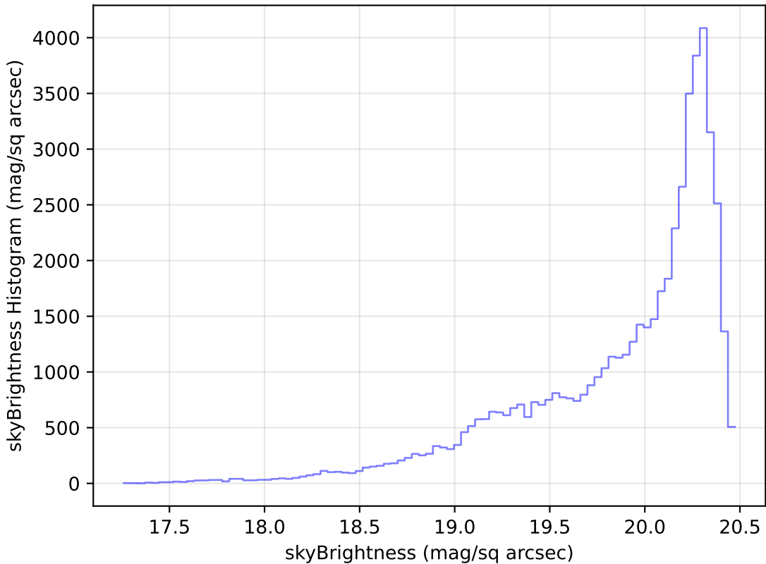
too_elab_r8_d2_griz_v3.4_10yrs Yr 1 i band: skyBrightness Histogram
