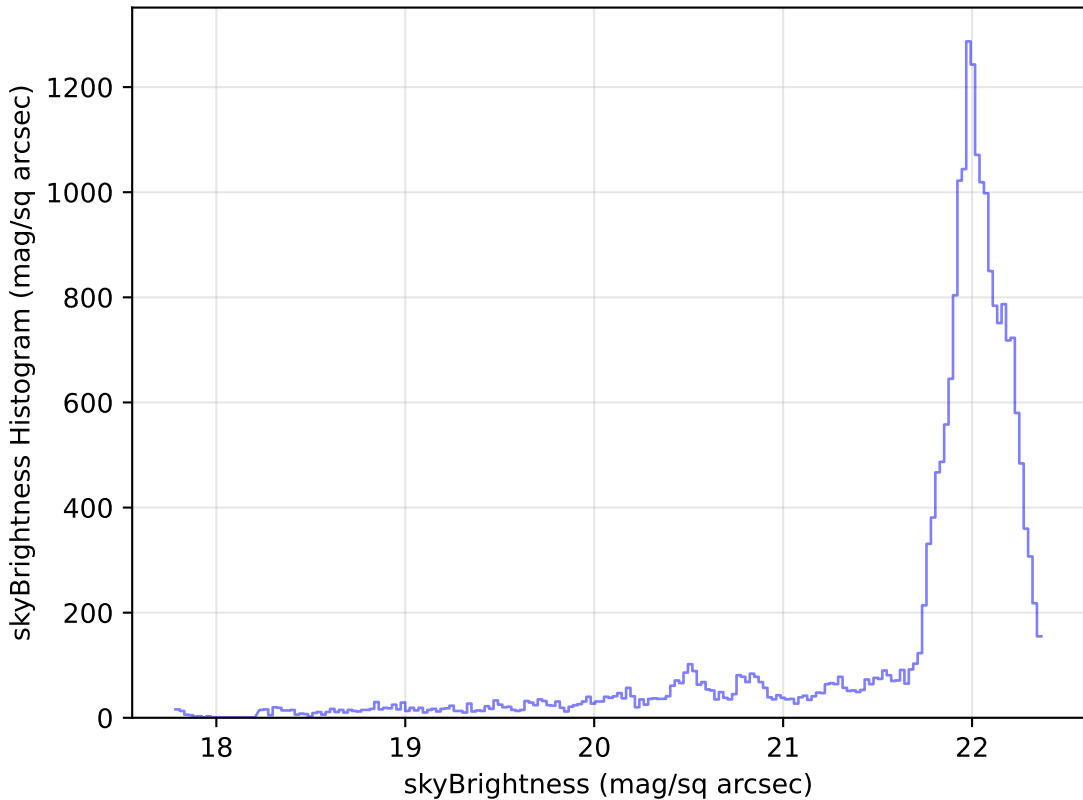
too_elab_r8_d2_griz_v3.4_10yrs Yr 1 g band: skyBrightness Histogram
