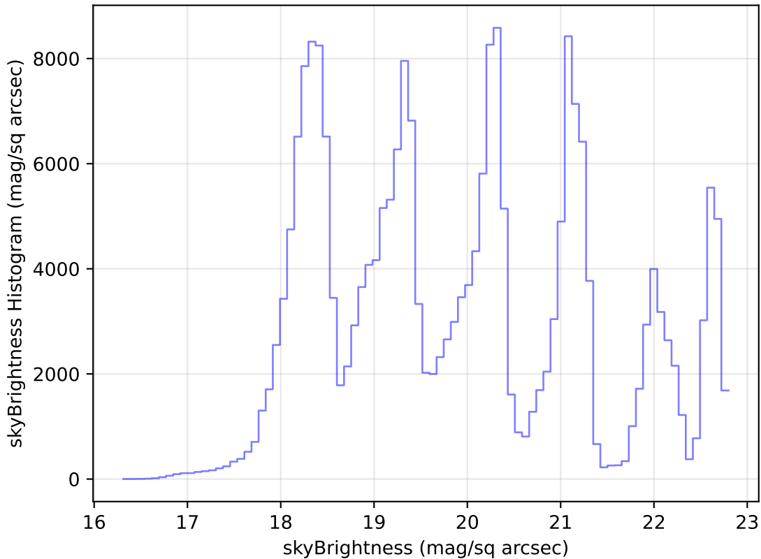
too_elab_r8_d2_griz_v3.4_10yrs Yr 1 all bands: skyBrightness Histogram
