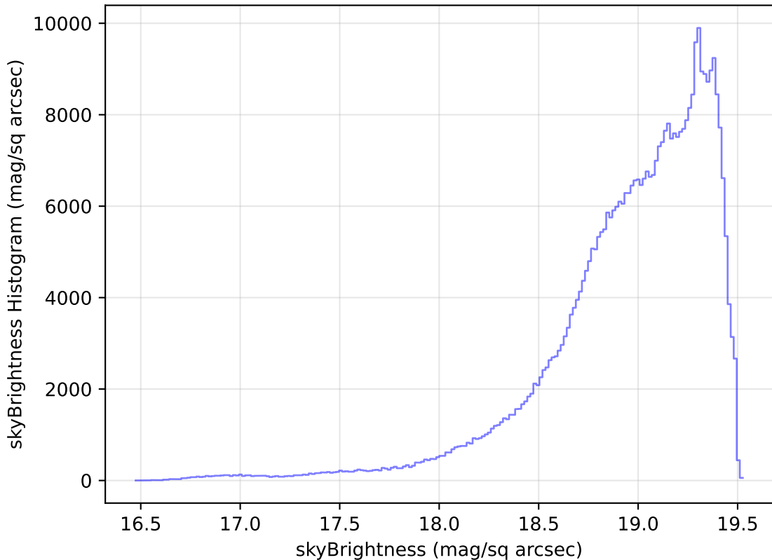
too_elab_r8_d2_griz_v3.4_10yrs WFD z band: skyBrightness Histogram
