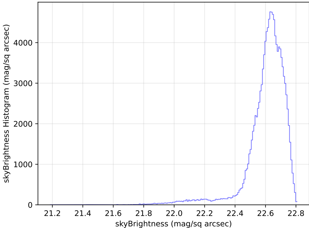
too_elab_r8_d2_griz_v3.4_10yrs WFD u band: skyBrightness Histogram
