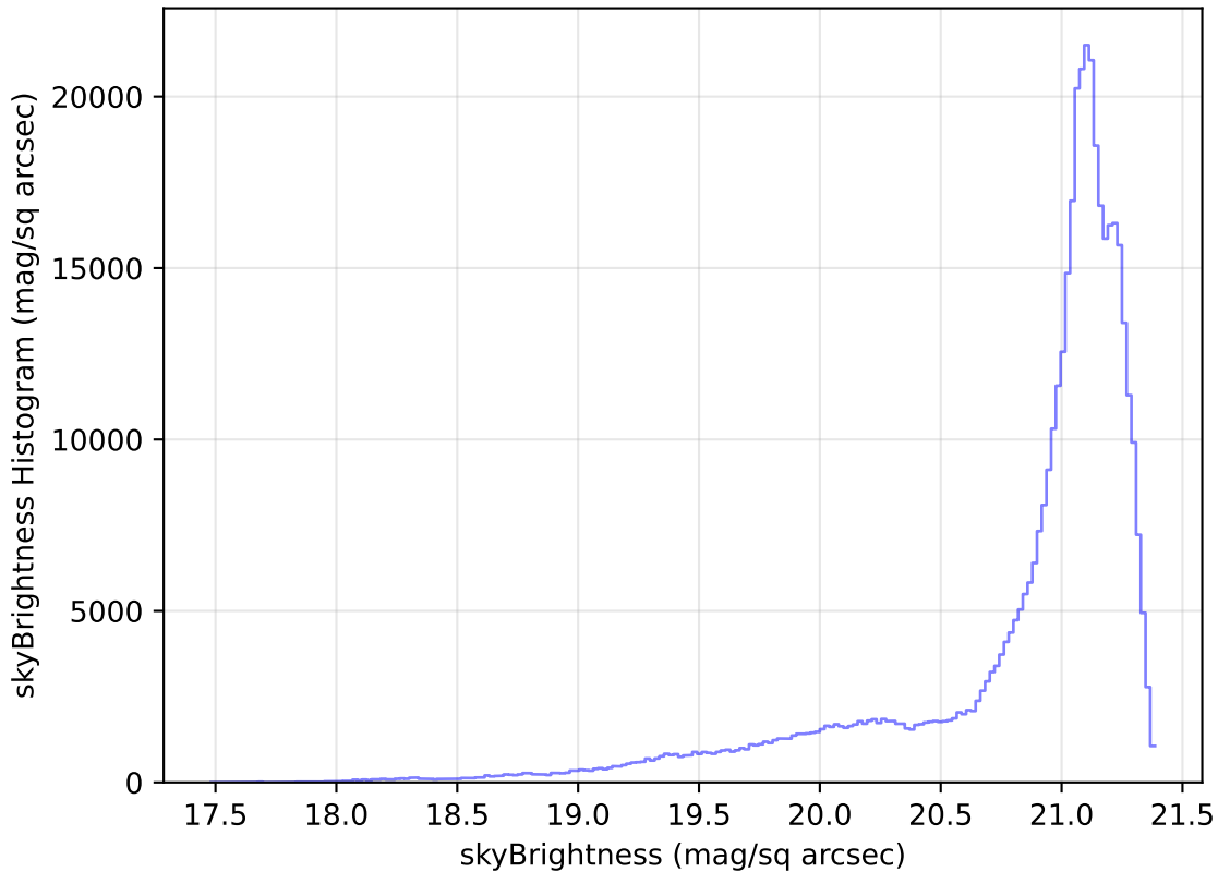
too_elab_r8_d2_griz_v3.4_10yrs WFD r band: skyBrightness Histogram
