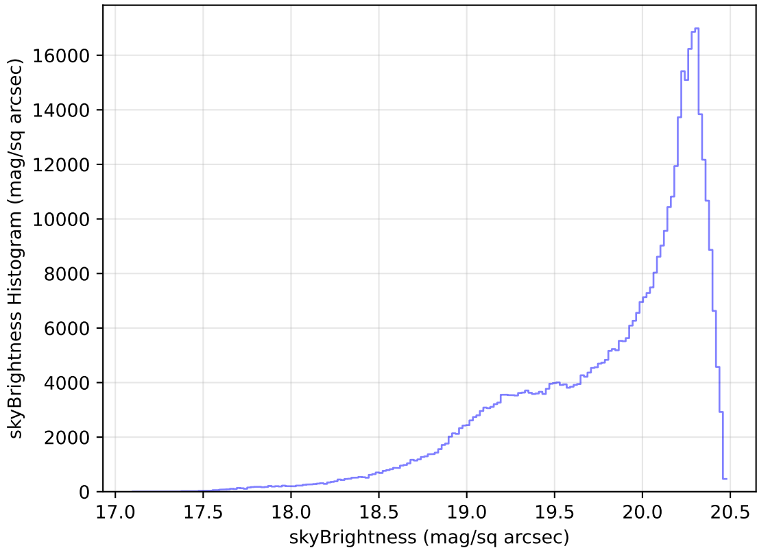
too_elab_r8_d2_griz_v3.4_10yrs WFD i band: skyBrightness Histogram
