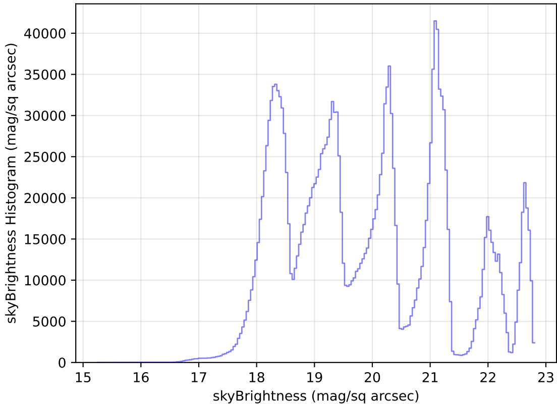
too_elab_r8_d2_griz_v3.4_10yrs WFD all bands: skyBrightness Histogram
