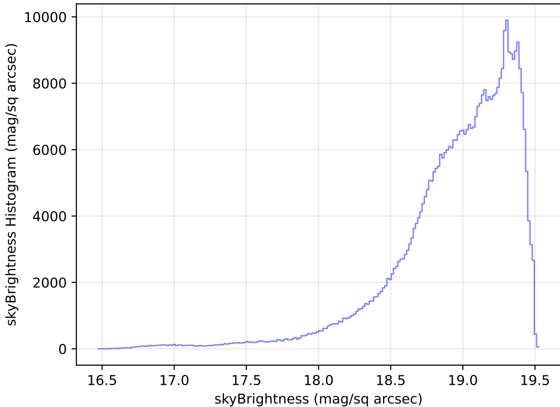
too_elab_r8_d2_griz_v3.4_10yrs All sky z band: skyBrightness Histogram
