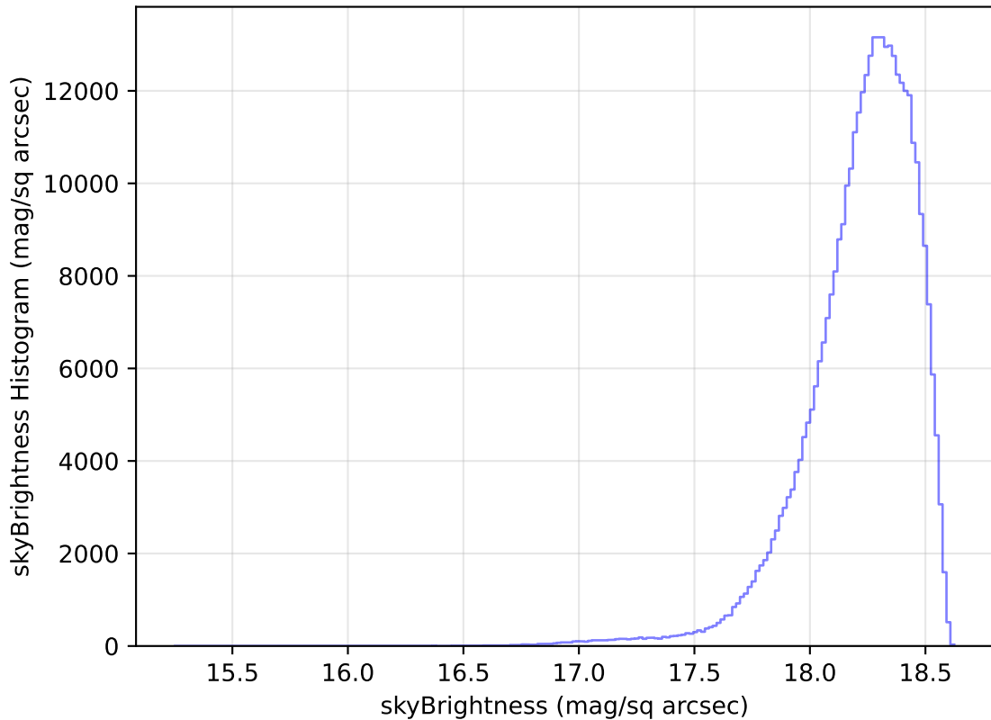
too_elab_r8_d2_griz_v3.4_10yrs All sky y band: skyBrightness Histogram
