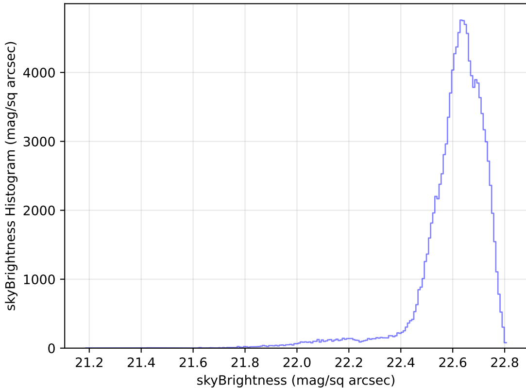
too_elab_r8_d2_griz_v3.4_10yrs All sky u band: skyBrightness Histogram
