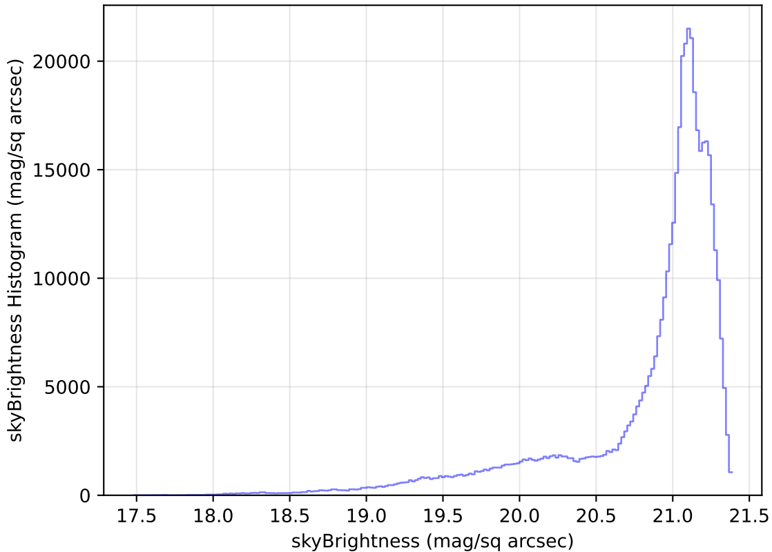
too_elab_r8_d2_griz_v3.4_10yrs All sky r band: skyBrightness Histogram
