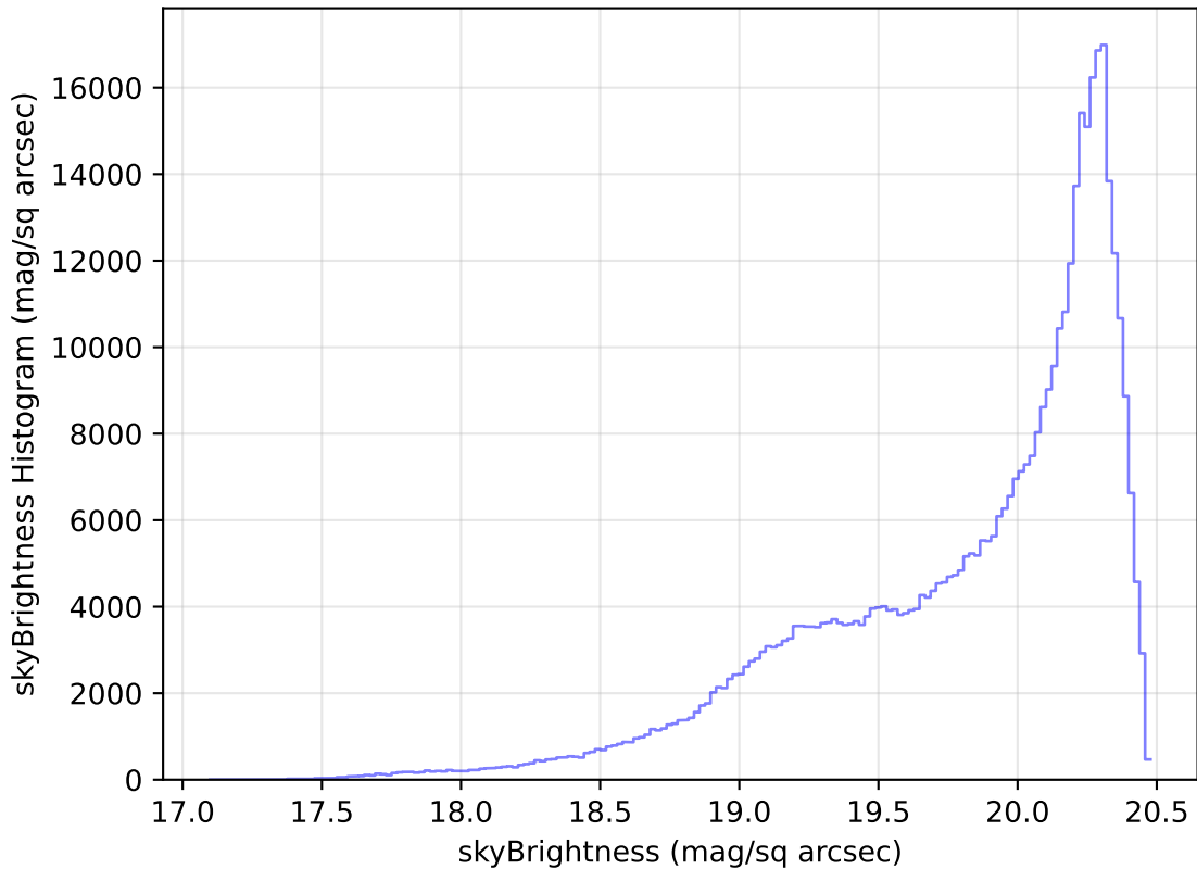
too_elab_r8_d2_griz_v3.4_10yrs All sky i band: skyBrightness Histogram
