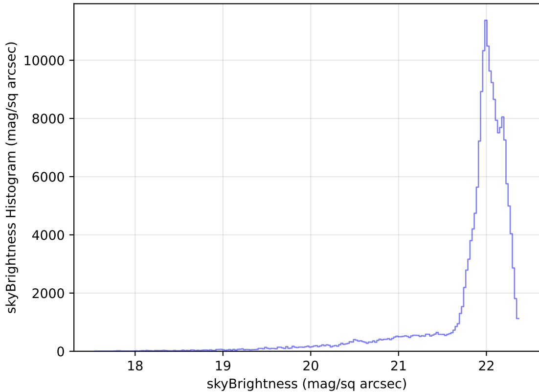
too_elab_r8_d2_griz_v3.4_10yrs All sky g band: skyBrightness Histogram
