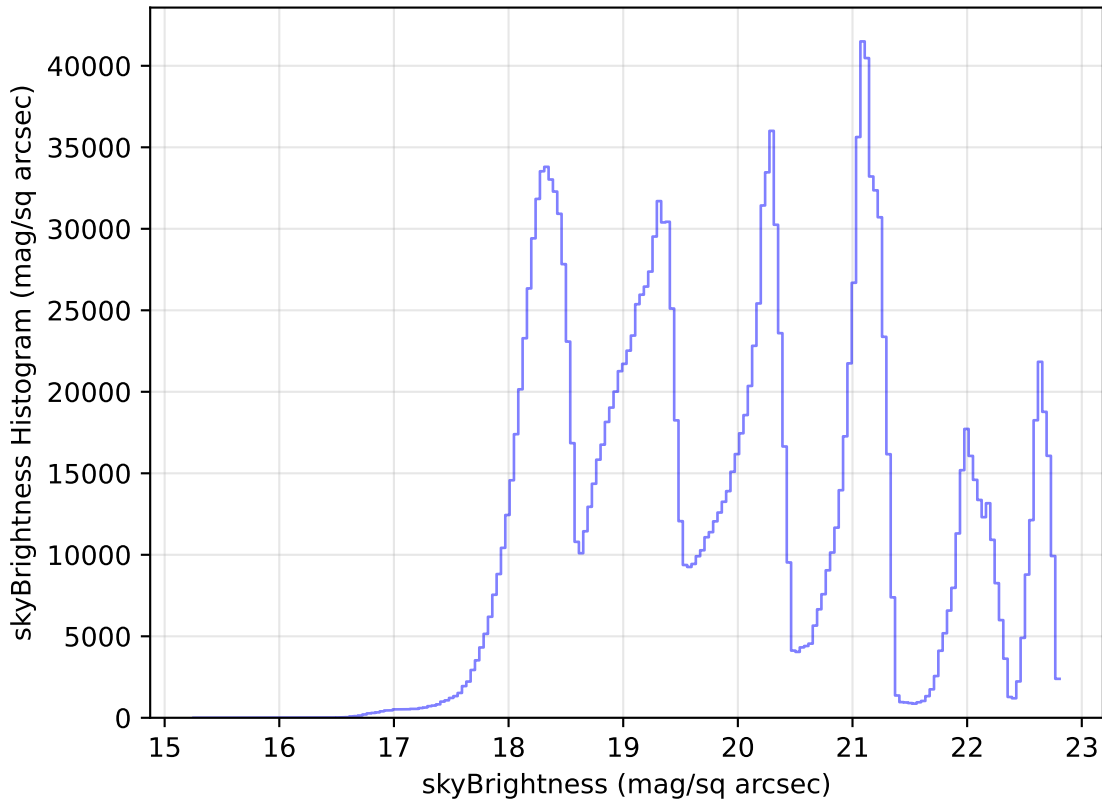
too_elab_r8_d2_griz_v3.4_10yrs All sky all bands: skyBrightness Histogram
