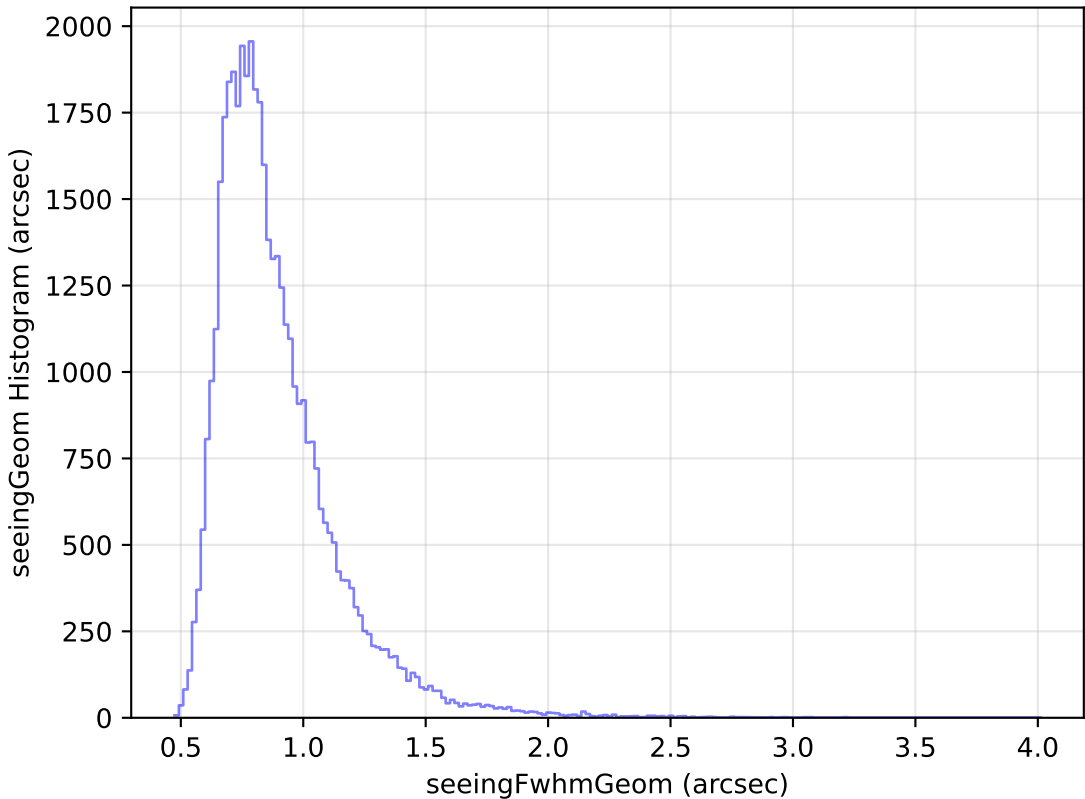
too_elab_r8_d2_griz_v3.4_10yrs Yr 1 z band: seeingGeom Histogram
