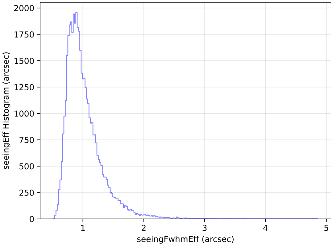
too_elab_r8_d2_griz_v3.4_10yrs Yr 1 z band: seeingEff Histogram
