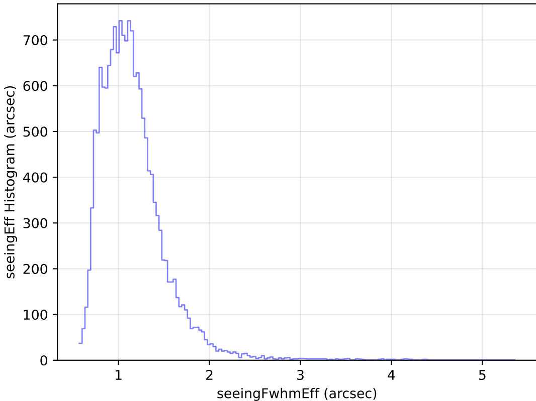
too_elab_r8_d2_griz_v3.4_10yrs Yr 1 u band: seeingEff Histogram
