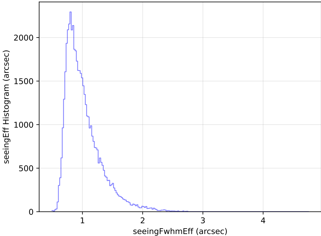
too_elab_r8_d2_griz_v3.4_10yrs Yr 1 r band: seeingEff Histogram
