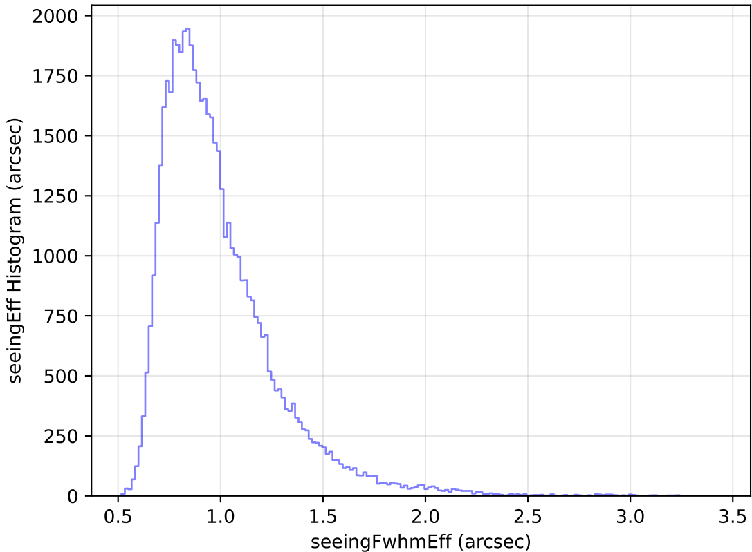
too_elab_r8_d2_griz_v3.4_10yrs Yr 1 i band: seeingEff Histogram
