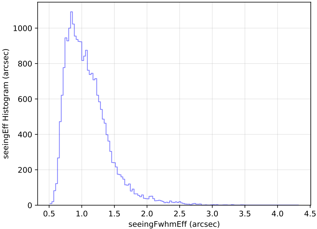
too_elab_r8_d2_griz_v3.4_10yrs Yr 1 g band: seeingEff Histogram
