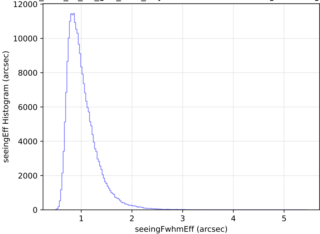
too_elab_r8_d2_griz_v3.4_10yrs Yr 1 all bands: seeingEff Histogram
