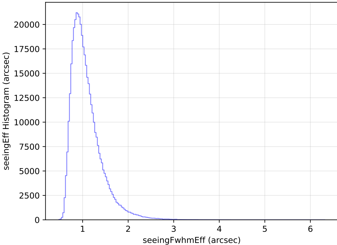
too_elab_r8_d2_griz_v3.4_10yrs WFD z band: seeingEff Histogram
