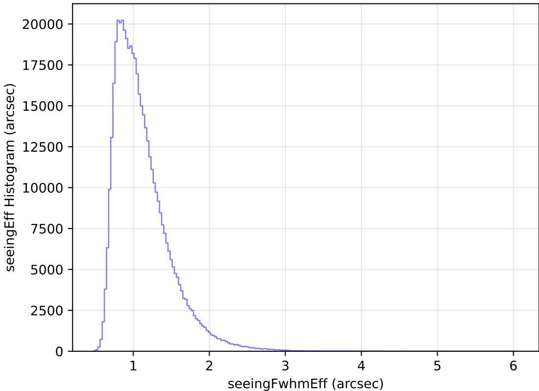
too_elab_r8_d2_griz_v3.4_10yrs WFD r band: seeingEff Histogram
