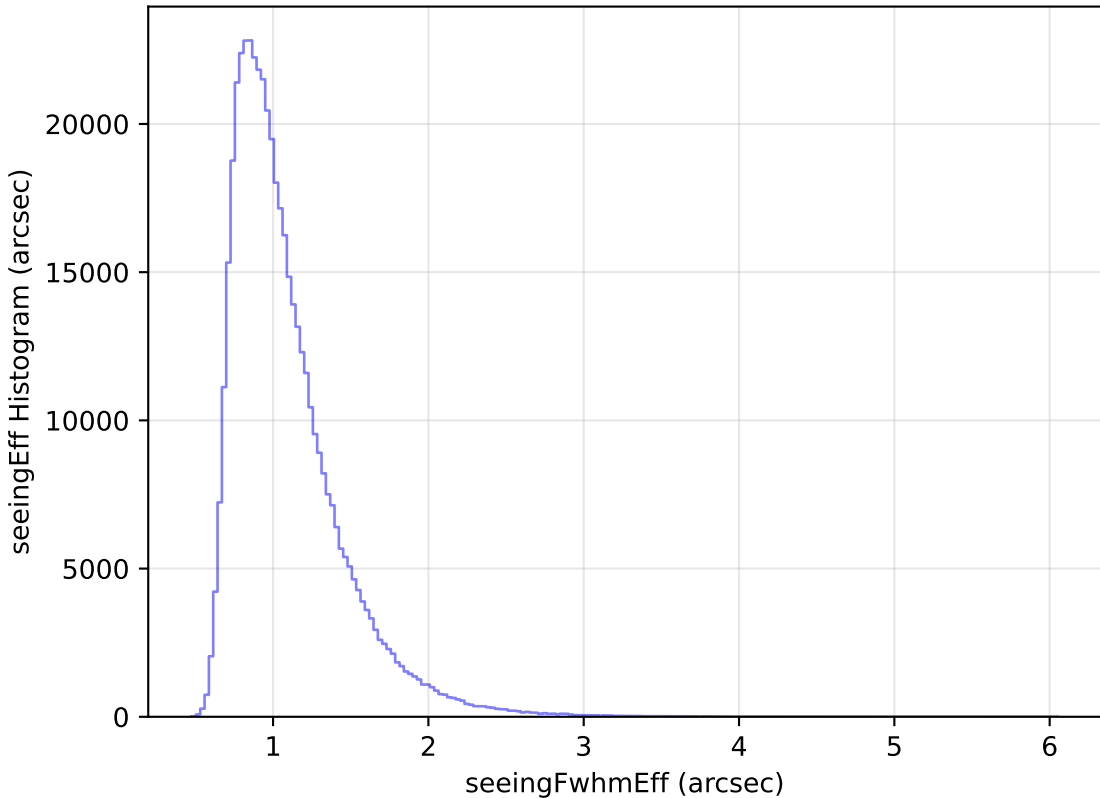
too_elab_r8_d2_griz_v3.4_10yrs WFD i band: seeingEff Histogram
