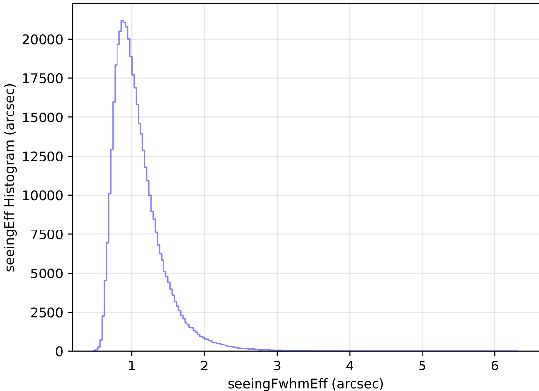
too_elab_r8_d2_griz_v3.4_10yrs All sky z band: seeingEff Histogram
