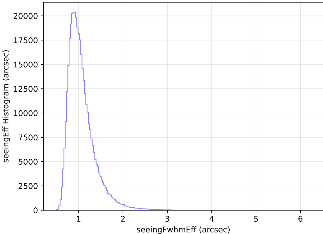
too_elab_r8_d2_griz_v3.4_10yrs All sky y band: seeingEff Histogram
