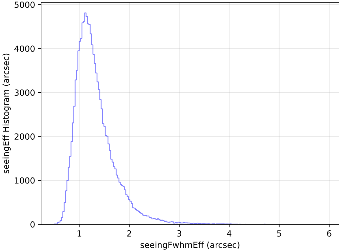
too_elab_r8_d2_griz_v3.4_10yrs All sky u band: seeingEff Histogram
