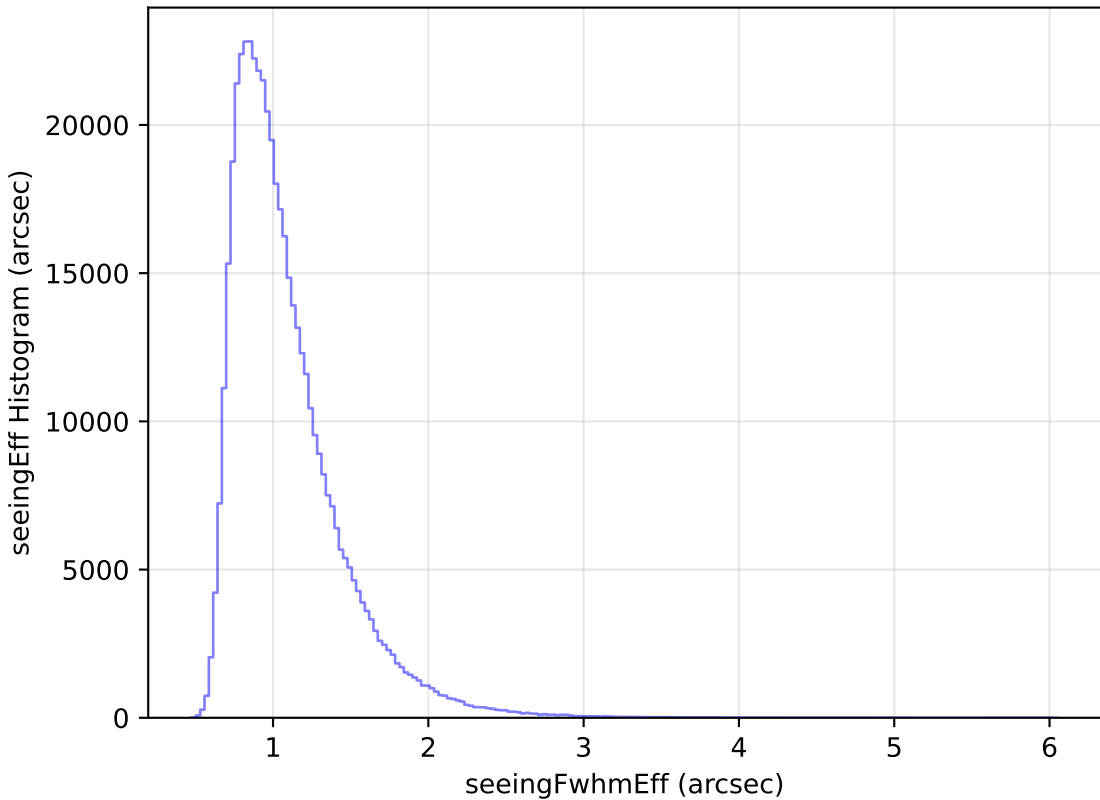
too_elab_r8_d2_griz_v3.4_10yrs All sky i band: seeingEff Histogram
