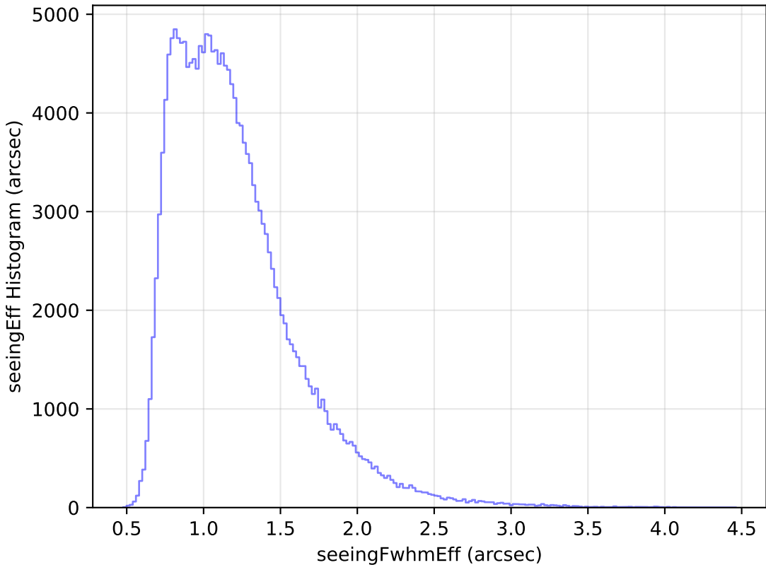
too_elab_r8_d2_griz_v3.4_10yrs All sky g band: seeingEff Histogram
