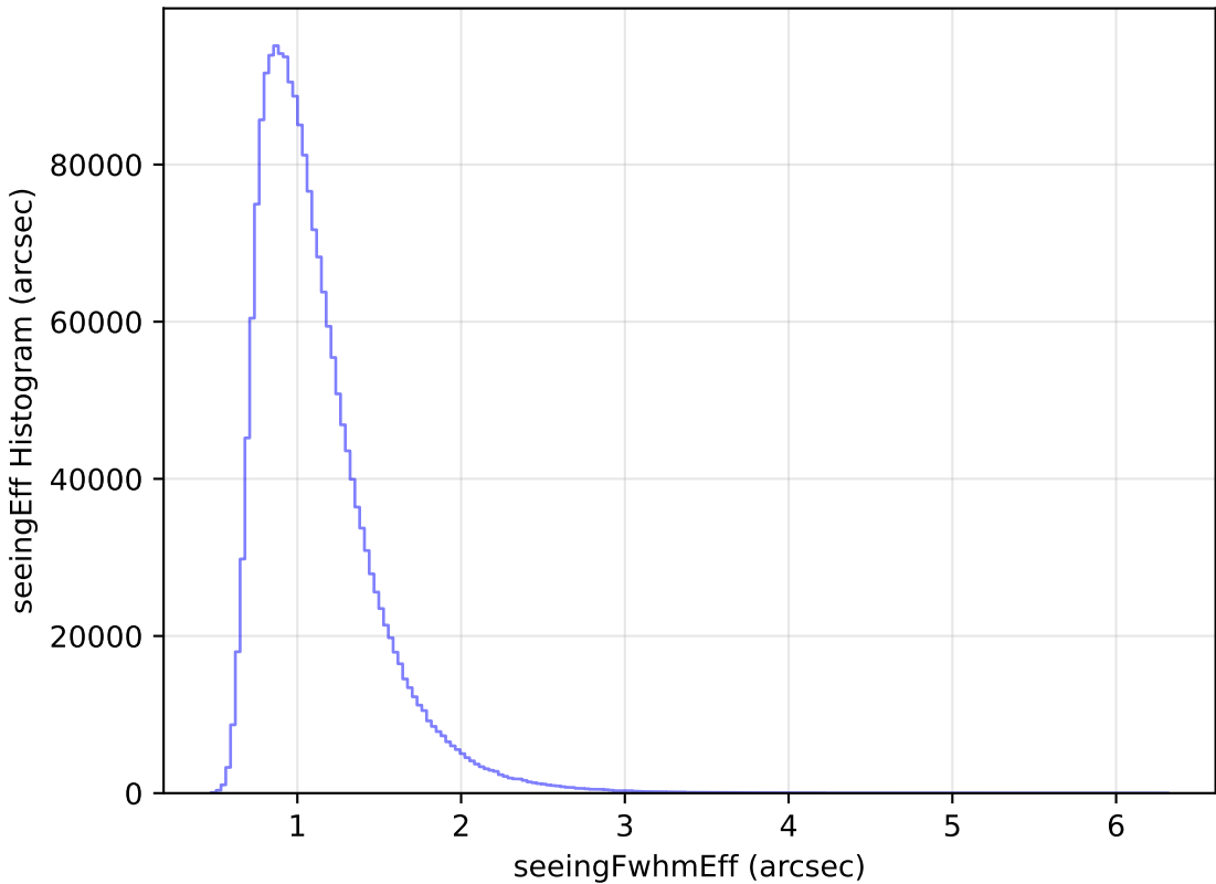
too_elab_r8_d2_griz_v3.4_10yrs All sky all bands: seeingEff Histogram
