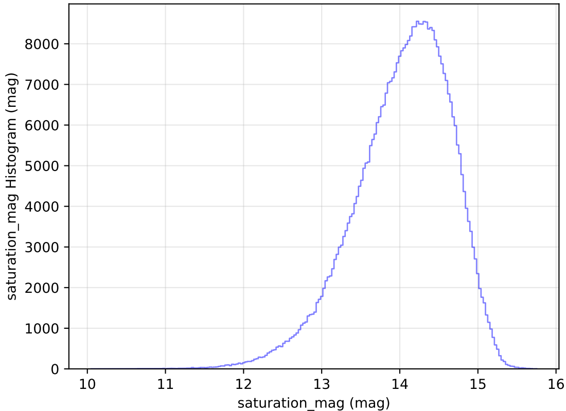
too_elab_r8_d2_griz_v3.4_10yrs WFD z band: saturation_mag Histogram
