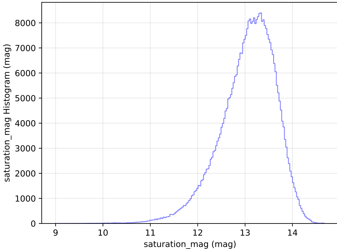
too_elab_r8_d2_griz_v3.4_10yrs WFD y band: saturation_mag Histogram
