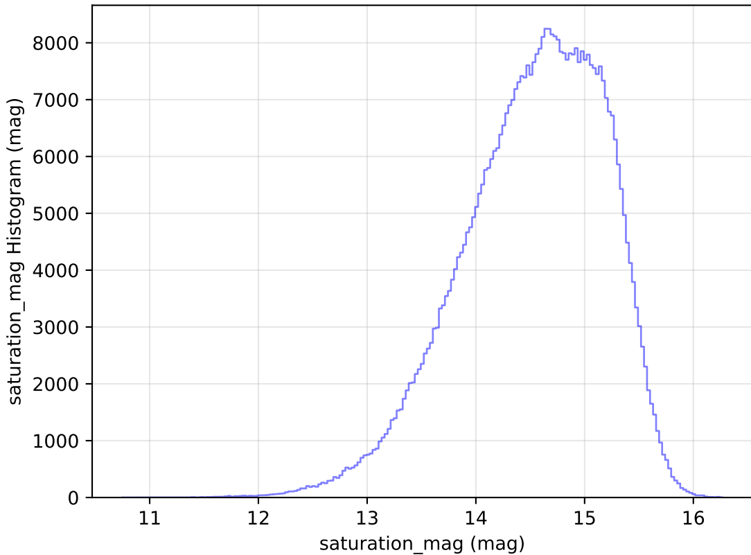
too_elab_r8_d2_griz_v3.4_10yrs WFD r band: saturation_mag Histogram
