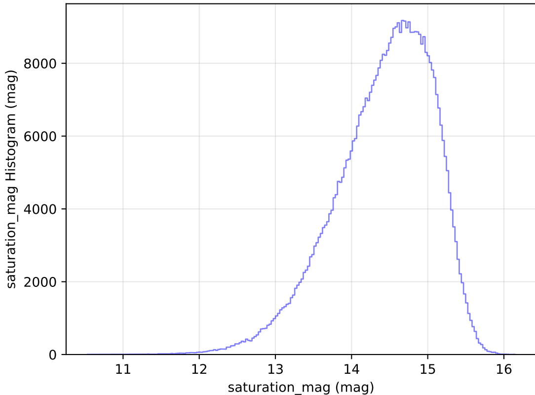
too_elab_r8_d2_griz_v3.4_10yrs WFD i band: saturation_mag Histogram
