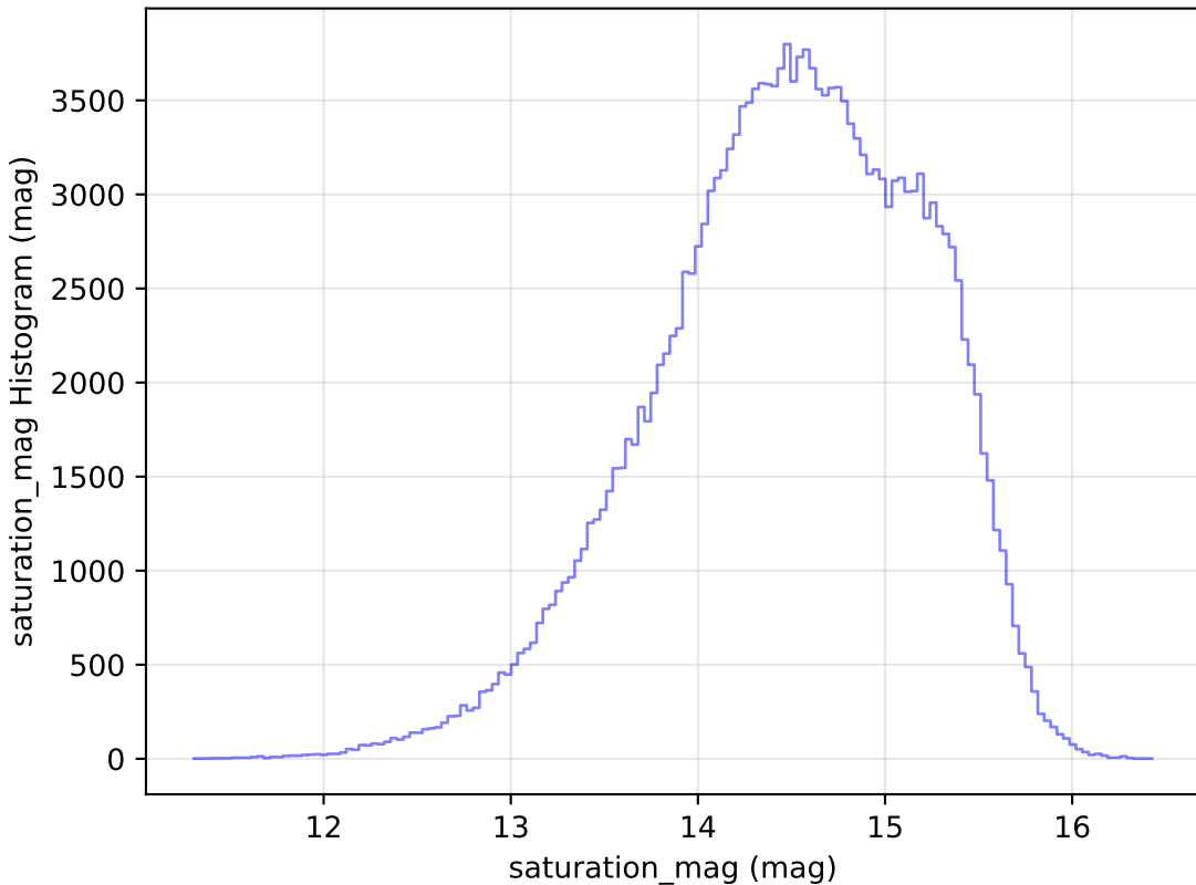
too_elab_r8_d2_griz_v3.4_10yrs WFD g band: saturation_mag Histogram
