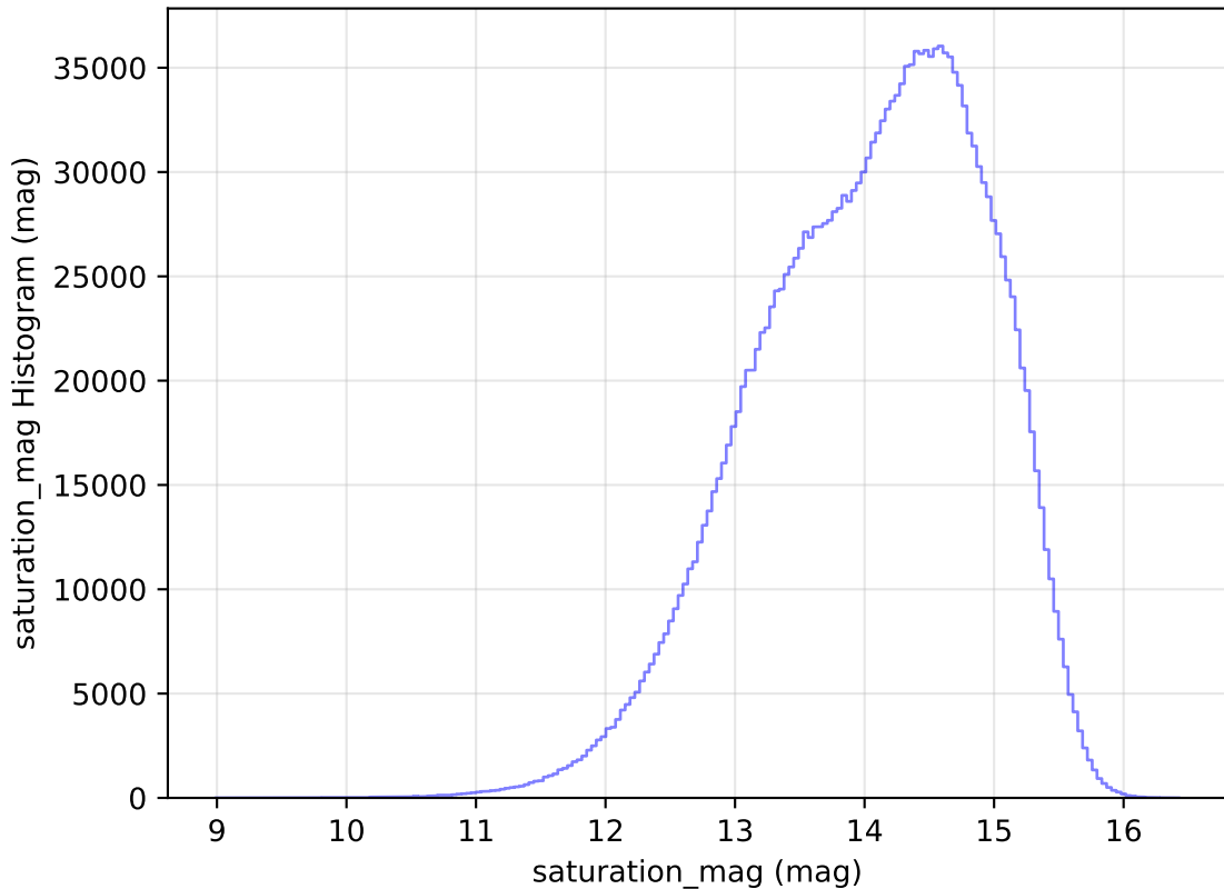
too_elab_r8_d2_griz_v3.4_10yrs WFD all bands: saturation_mag Histogram
