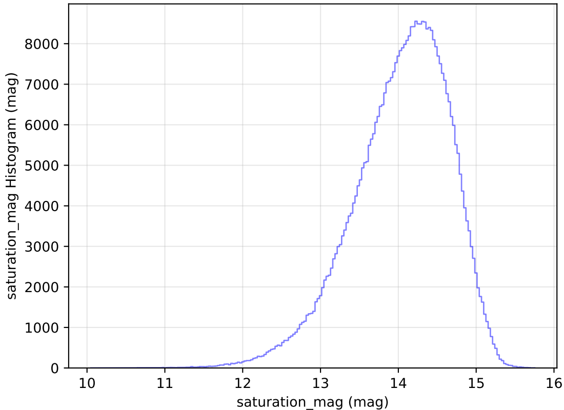
too_elab_r8_d2_griz_v3.4_10yrs All sky z band: saturation_mag Histogram
