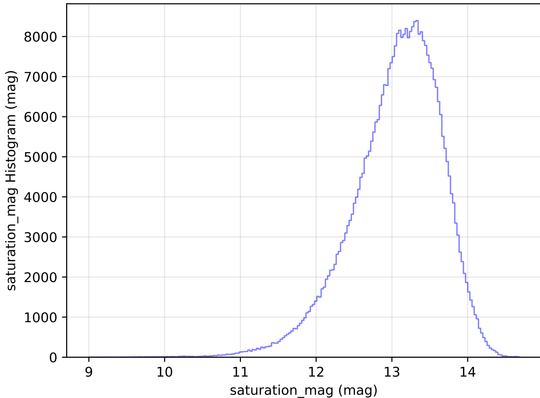
too_elab_r8_d2_griz_v3.4_10yrs All sky y band: saturation_mag Histogram
