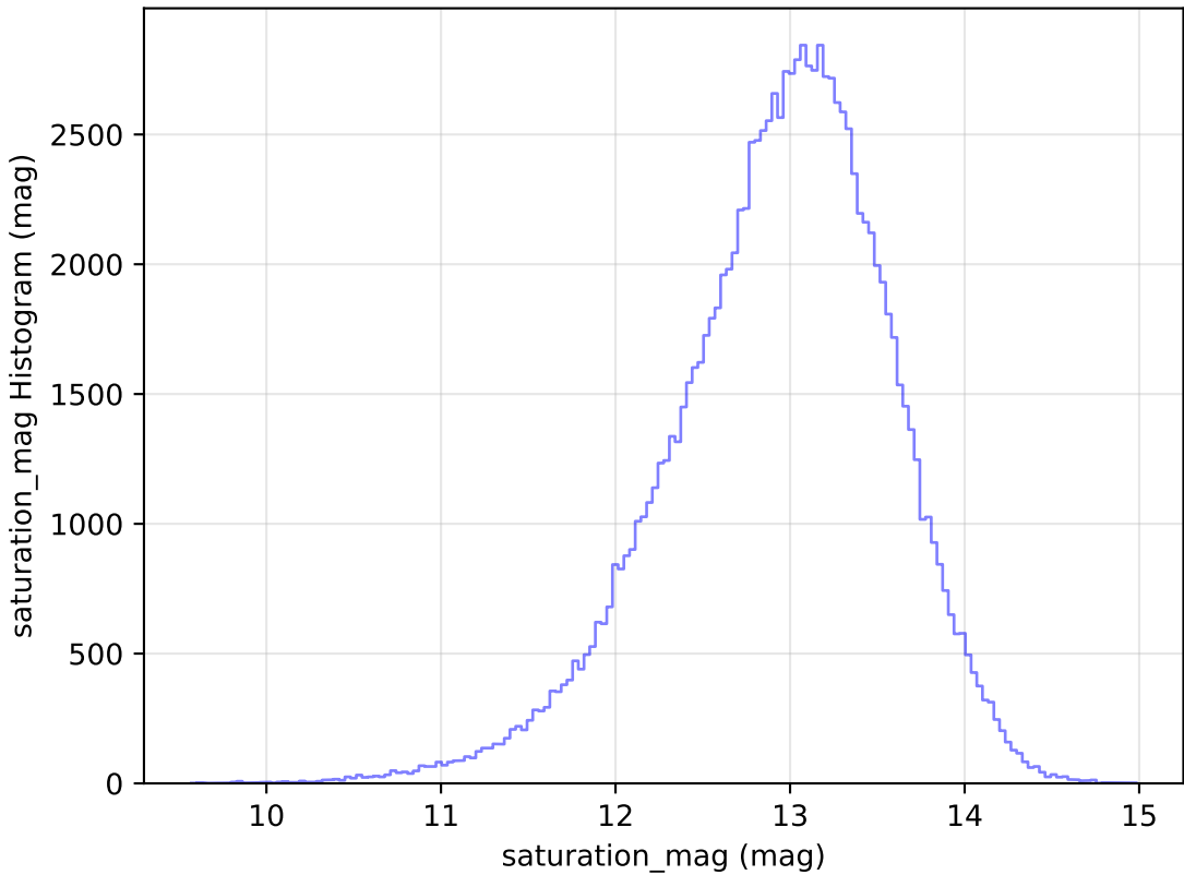
too_elab_r8_d2_griz_v3.4_10yrs All sky u band: saturation_mag Histogram
