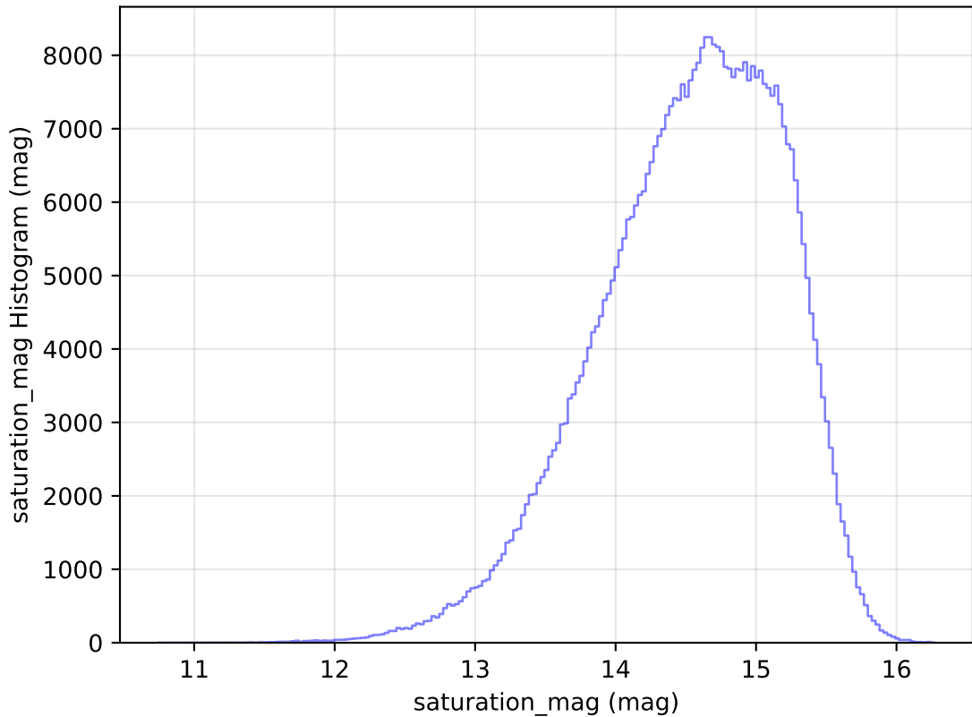
too_elab_r8_d2_griz_v3.4_10yrs All sky r band: saturation_mag Histogram
