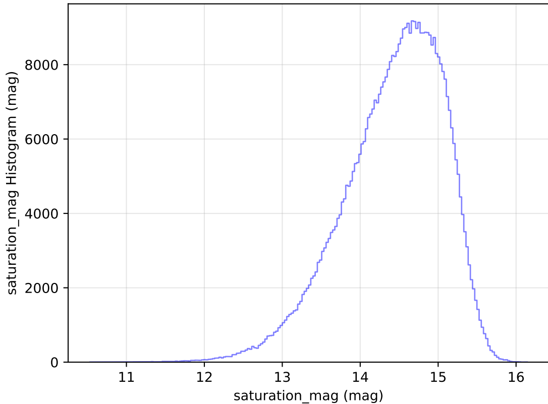
too_elab_r8_d2_griz_v3.4_10yrs All sky i band: saturation_mag Histogram
