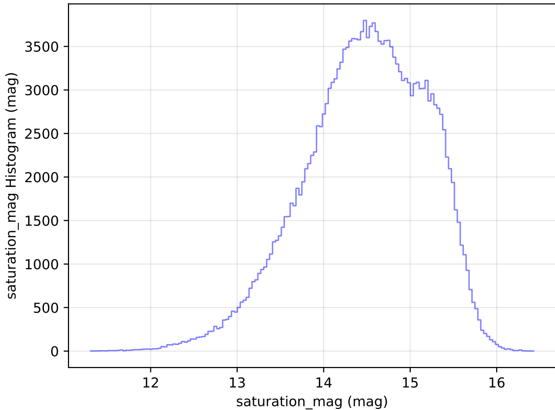
too_elab_r8_d2_griz_v3.4_10yrs All sky g band: saturation_mag Histogram
